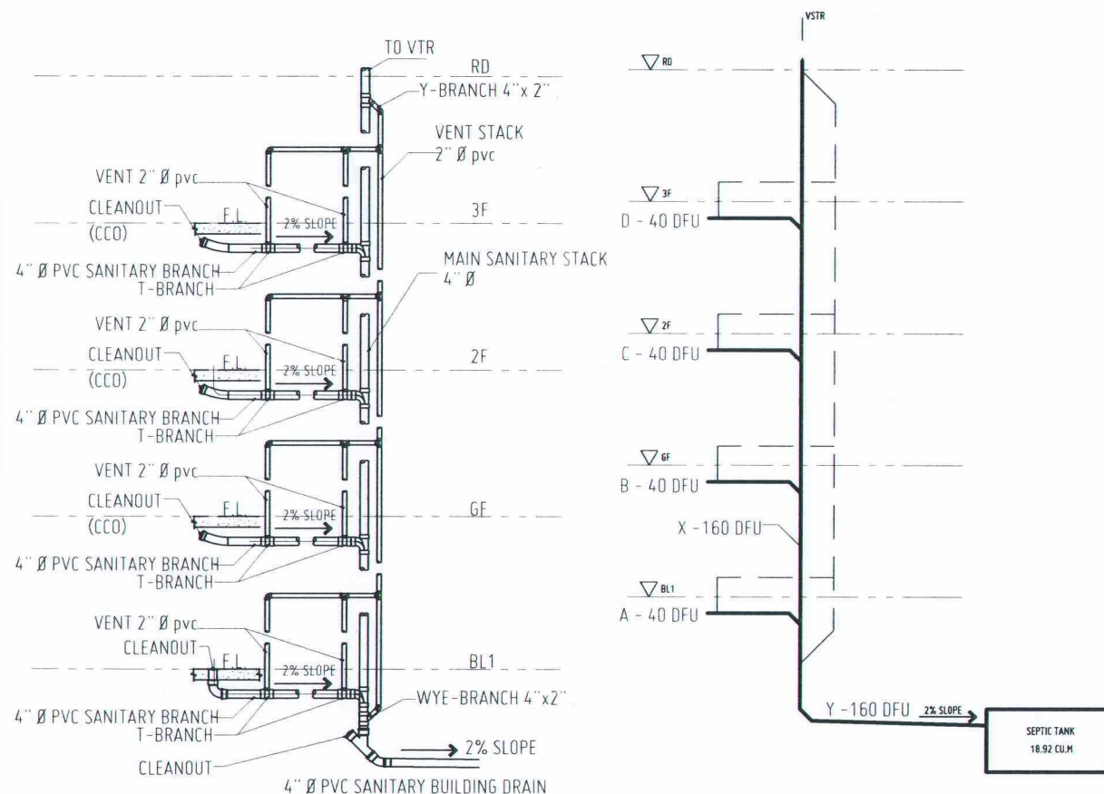
SOIL PIPE LINE RISER DIAGRAM SCALE: NDTs
