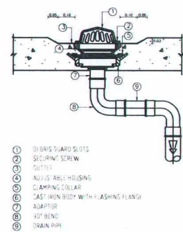
ROOF DRAIN
