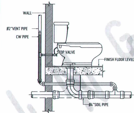
WATER CLOSET WITH FLUSH TANK (WC)
