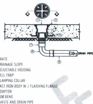
FLOOR DRAIN (USE FOR SLAB ON GROUND)
