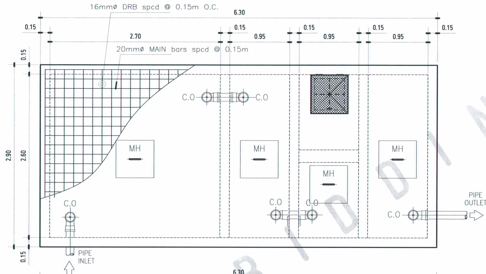
P 16 1 BLOW-UP PLAN DETAIL
