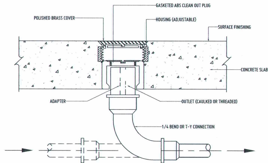
FLOOR CLEANOUT
