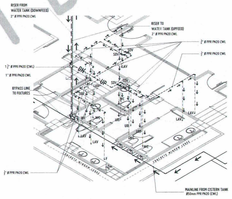
P 10 7 BLOWUP - WATERLINE ISOMETRIC VIEW ZONE 1 GROUND FLOOR - PUBLIC TOILETS SCALE: NTS
