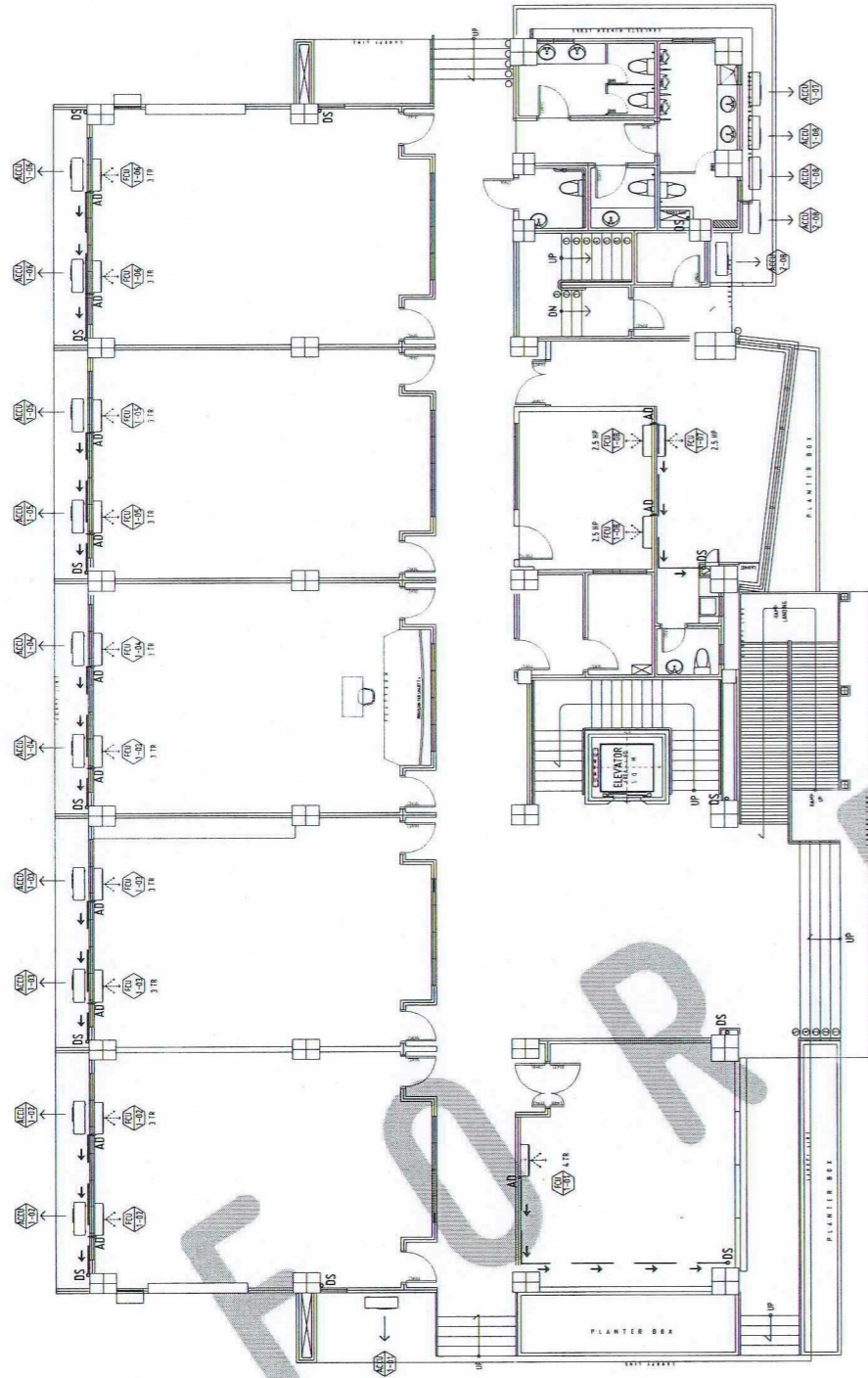
AIRCON DRAIN LAYOUT PLAN
