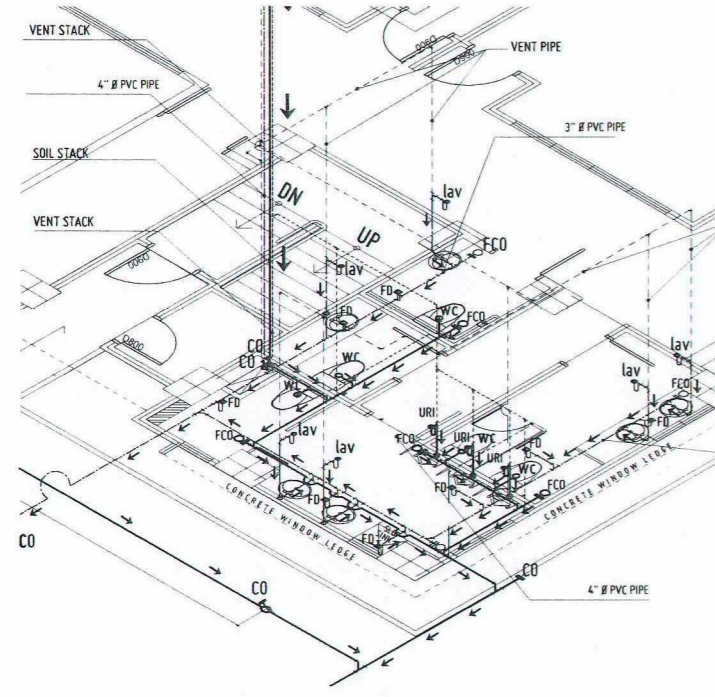
P 10 1 BLOWUP - SOIL & WASTE ISOMETRIC VIEW ZONE 1 GROUND FLOOR - PUBLIC TOILETS SCALE: NTS
