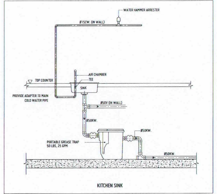
P 11 5 PORTABLE GREASE TRAP CONNECTION SCALE: 1:10 MTS
