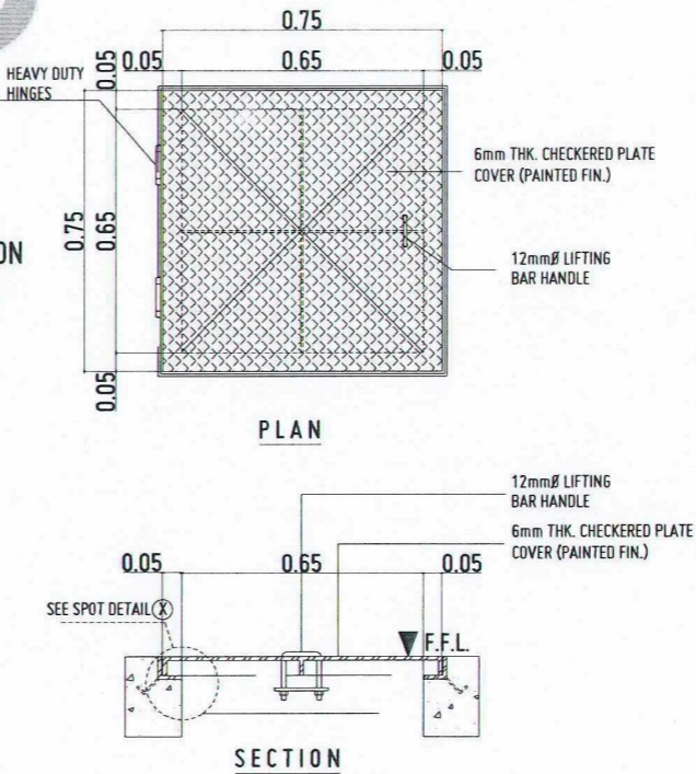
P 11 6 METAL MANHOLE COVER DETAIL SCALE: 1:10 MTS
