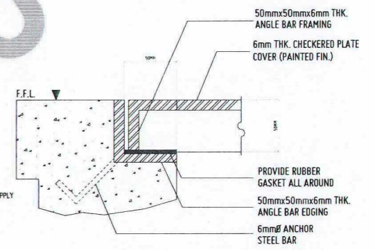
P 11 4 SPOT DETAIL "X" SCALE: NTS
