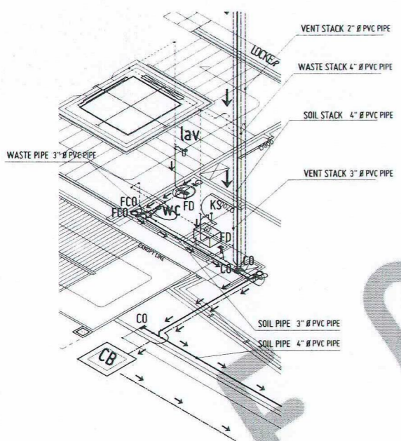
P 10 3 BLOWUP - SOIL & WASTE ISOMETRIC VIEW ZONE 2 GROUND FLOOR - OFFICE TOILET SCALE: NTS
