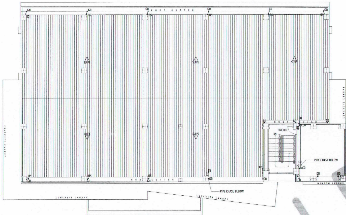
P 6 1 ROOF DECK - STORM DRAIN LAYOUT SCALE: 1:100 MTS
