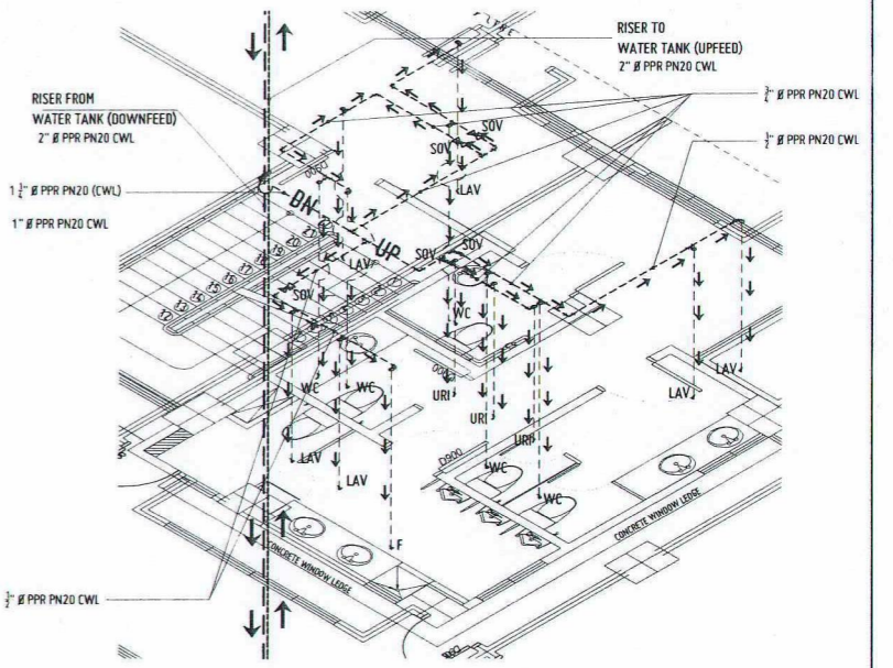
P 10 8 TYPICAL BLOWUP - WATERLINE ISOMETRIC VIEW ZONE 1 2ND FLR TO 5TH FLR - PUBLIC TOILETS SCALE: NTS
