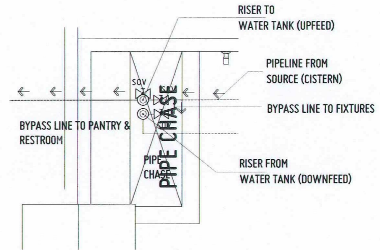
P 6 4 SPOT DETAIL W2 SCALE: 1:10 MTS
