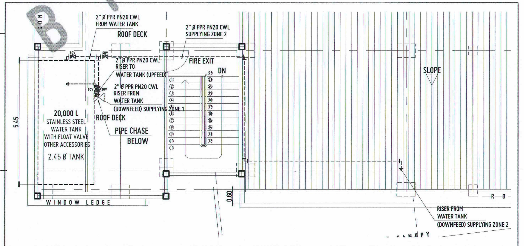
BLOW-UP PLAN ZONE 1
