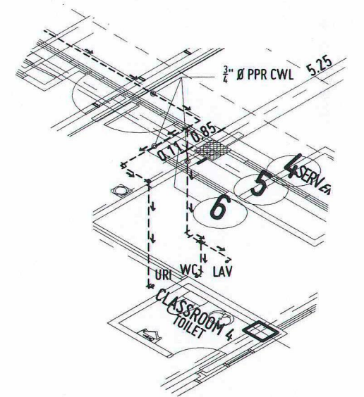
WATERLINE PIPING LAYOUT
