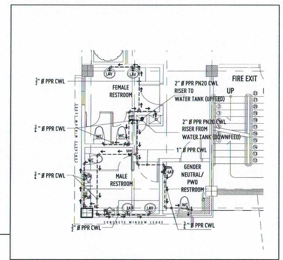
TYPICAL BLOW-UP PLAN 2ND & 3RD FLR - ZONE 1 SCALE: 1:100 MTS
