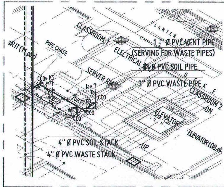
TYPICAL BLOW-UP ISOMETRIC VIEW
