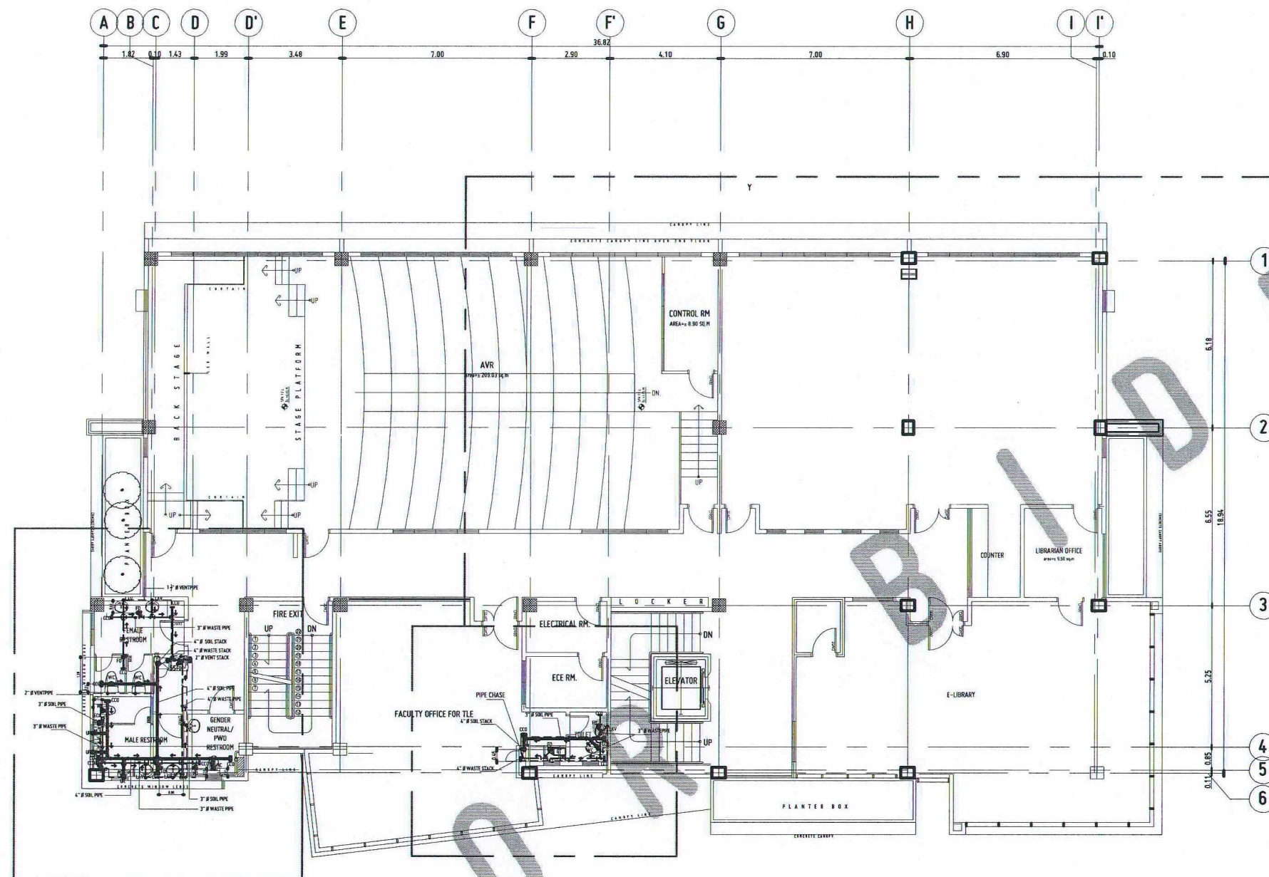
INDEX PLAN THIRD FLOOR
