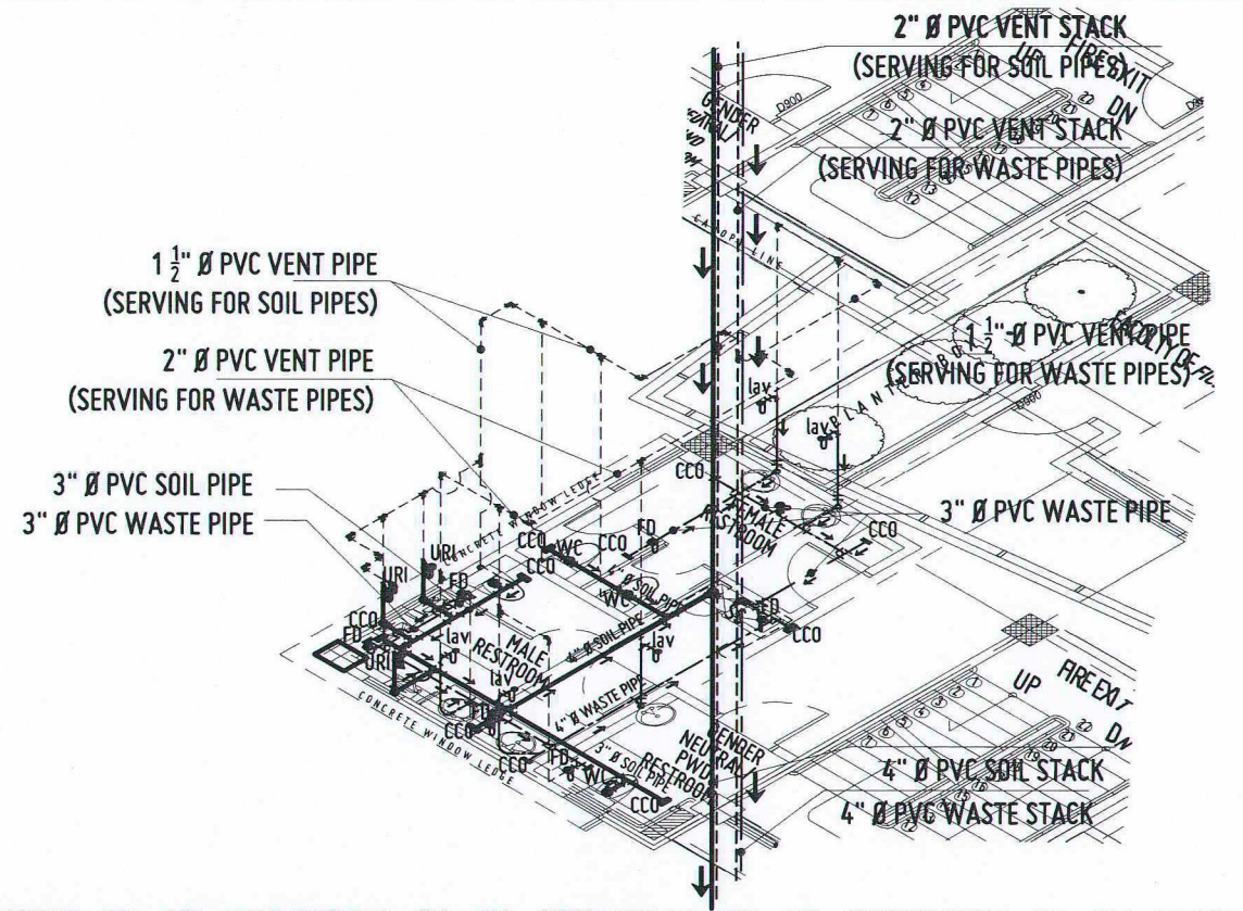
TYPICAL BLOW-UP ISOMETRIC VIEW
