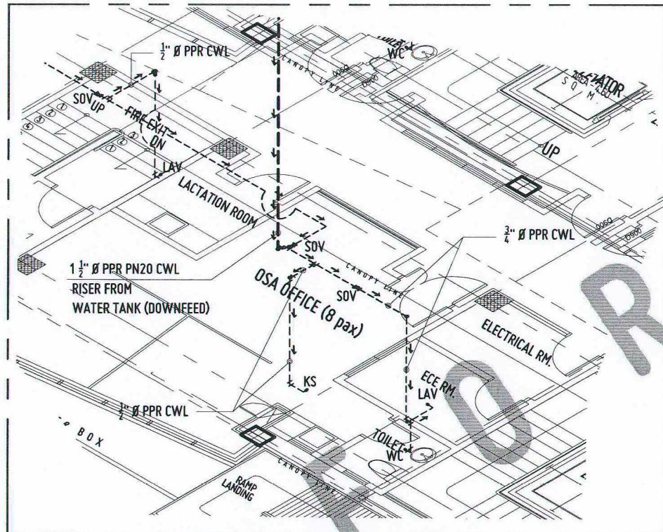
BLOW-UP ISOMETRIC VIEW
