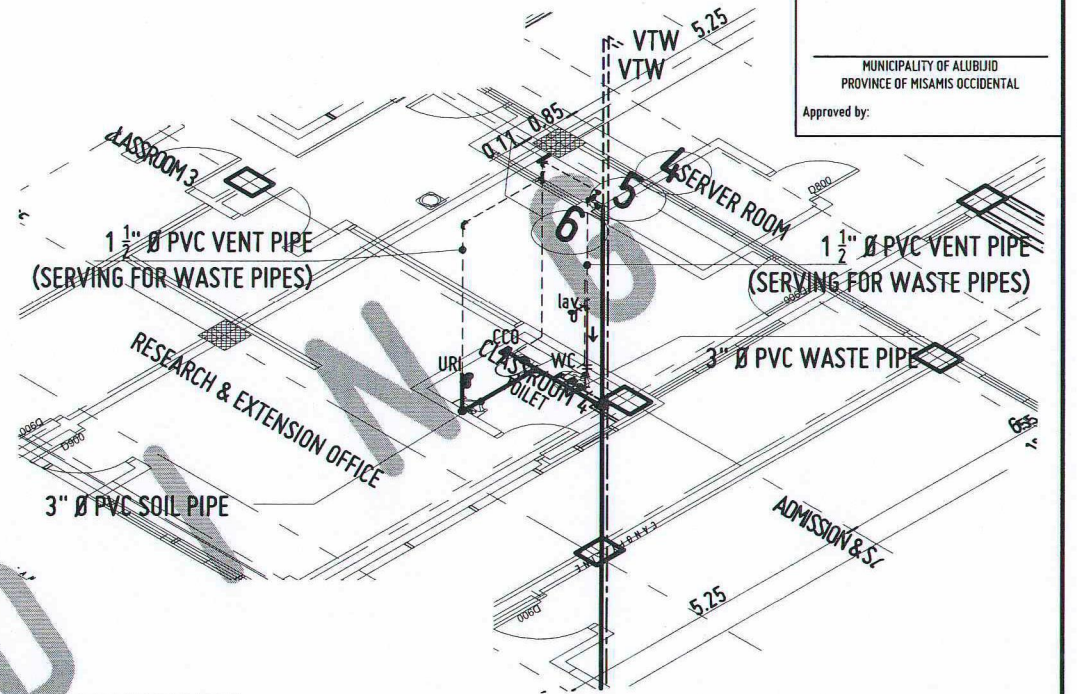
SOIL & WASTE PIPING LAYOUT
