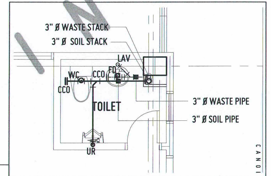
BLOW-UP PLAN RESEARCH & EXTENSION OFFICE RESTROOM SCALE: 1:50 MTS
