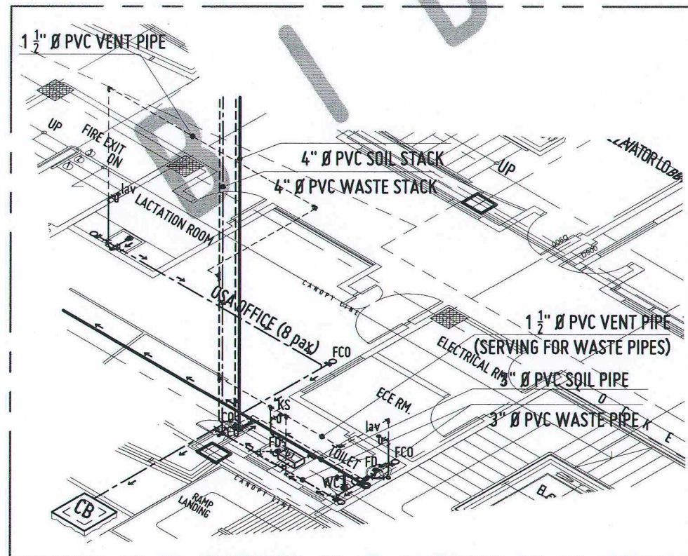
BLOW-UP ISOMETRIC VIEW
