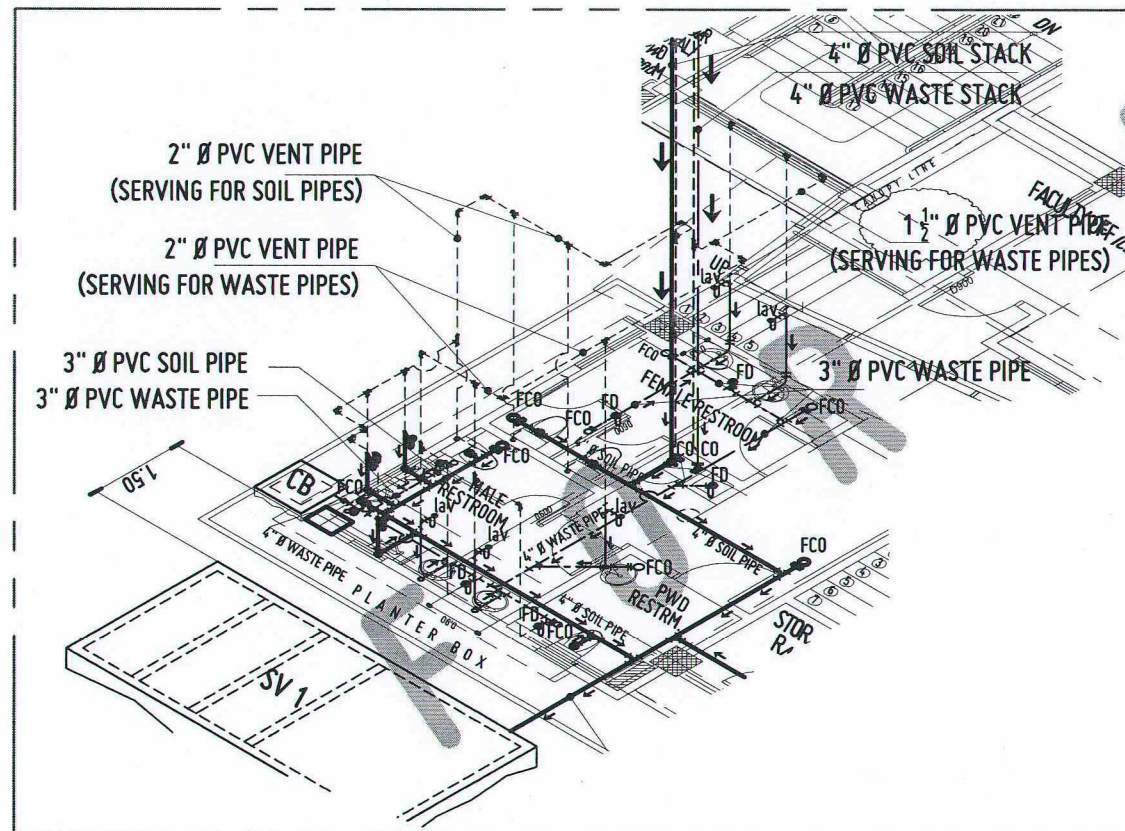
BLOW-UP ISOMETRIC VIEW
