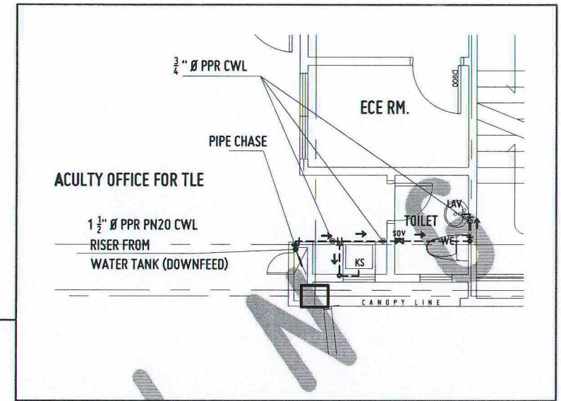
TYPICAL BLOW-UP PLAN 2ND & 3RD FLR - ZONE 2 SCALE: 1:100 MTS
