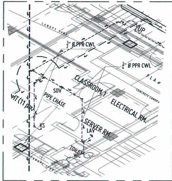
TYPICAL BLOW-UP ISOMETRIC VIEW
