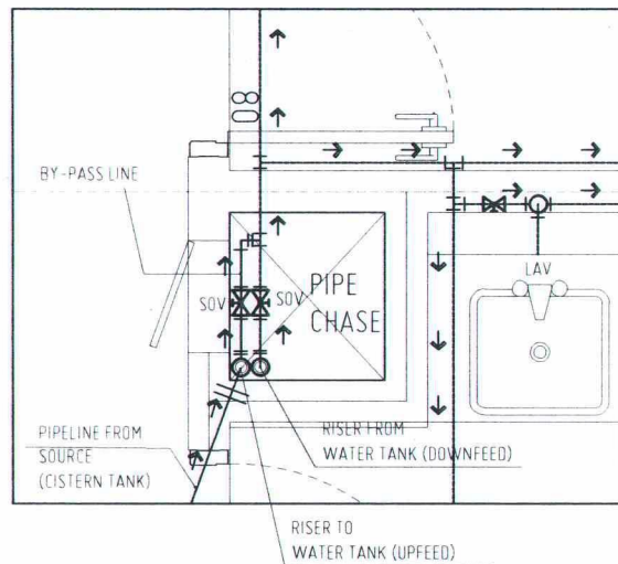
SPOT DETAIL "X" SCALE: 1:30 MTS
