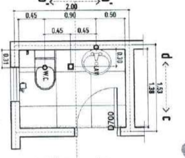
STUB-OUT PLAN STAFF/FACULTY RESTROOM SCALE: 1:30 MTS
