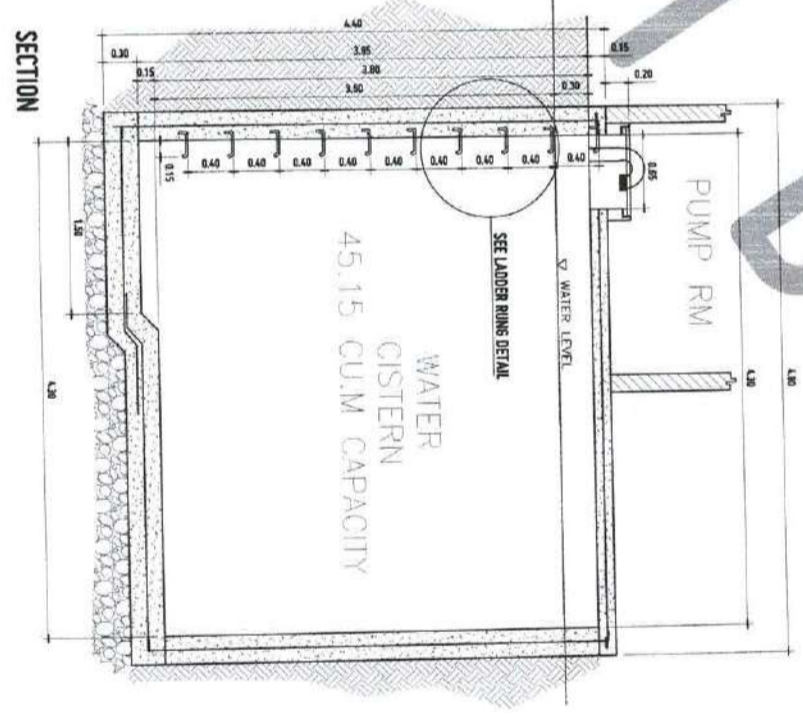
WATER CISTERN DETAIL SCALE: 1:30 MTS
