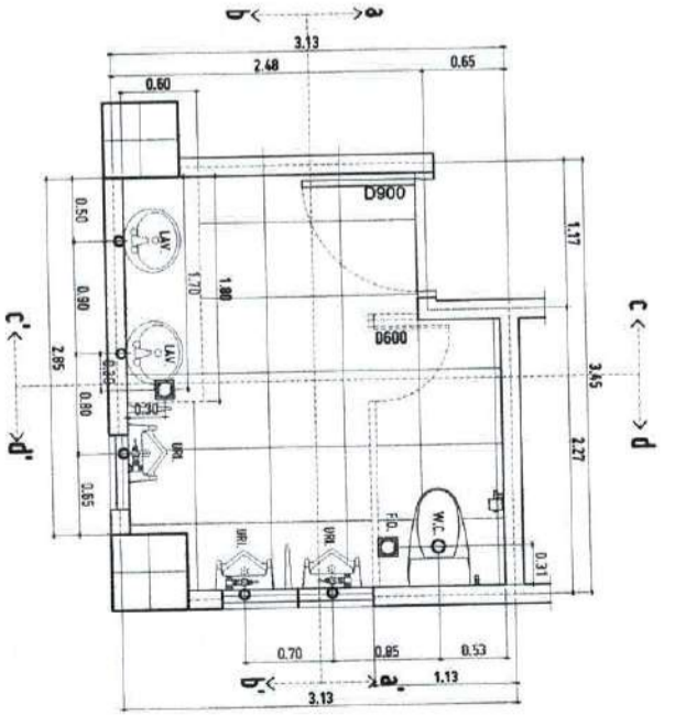
STUB-OUT PLAN MALE RESTROOM SCALE: 1:30 MTS
