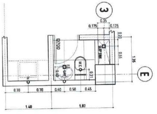
FIFTH FLOOR - WATER LINE LAYOUT - FUTURE DEVELOPMENT SCALE: 1:100 MTS
