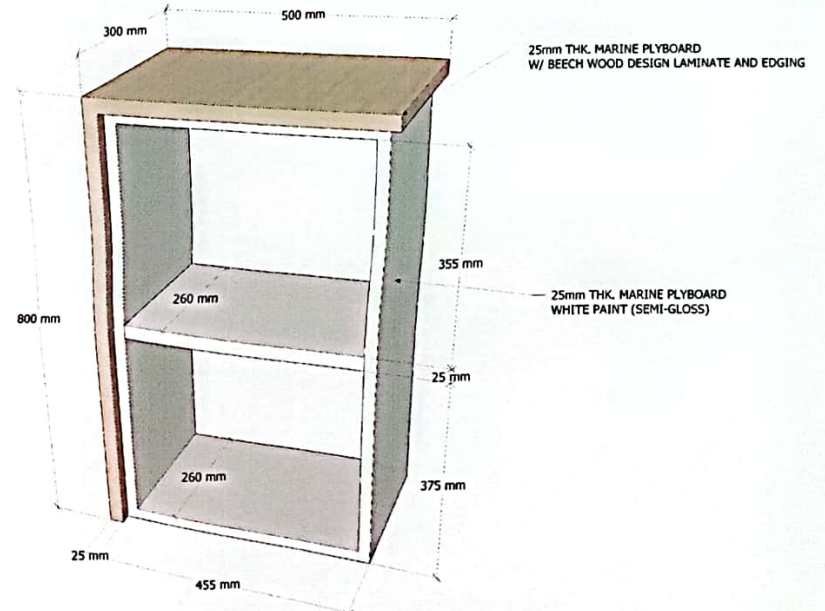
3 SIDE TABLE DETAIL (40 SETS) SCALE: A/44
