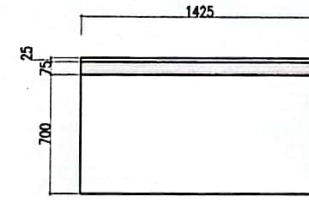
4 NOOK FRONT VIEW A/32
