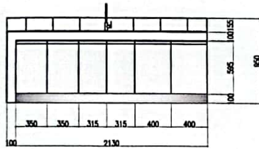
1 LEFT SIDE VIEW A33
