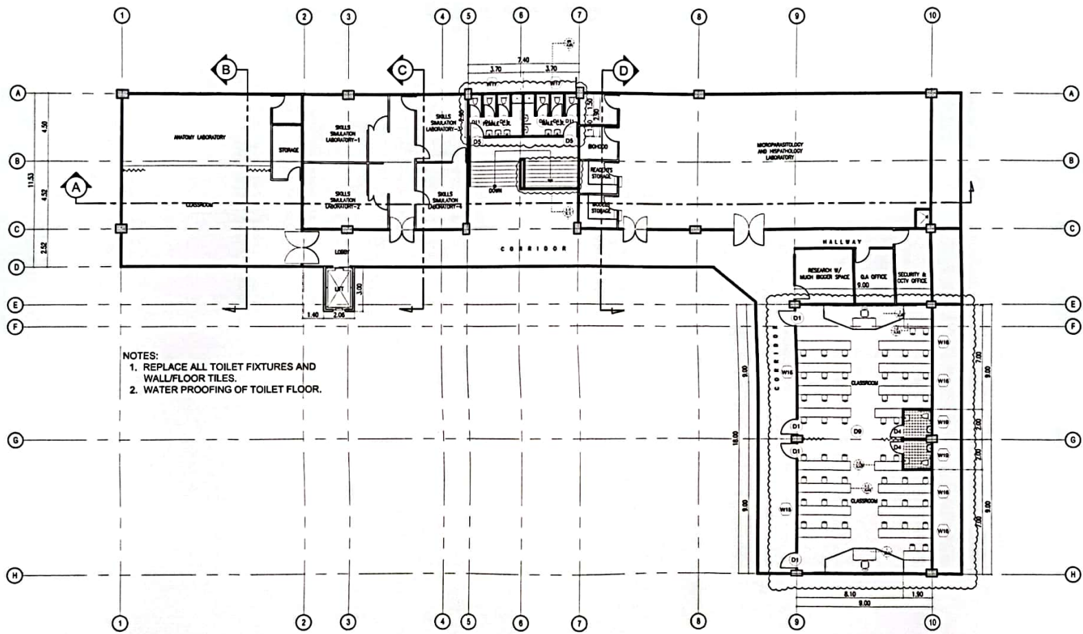
1 A/13 PROPOSED SECOND FLOOR PLAN SCALE: 1:200M
