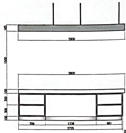
2 FRONT VIEW A/30
