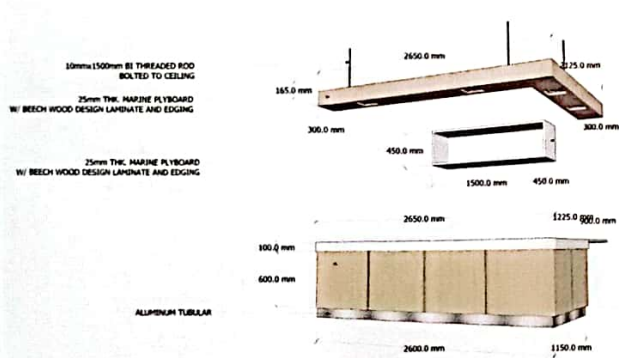
6 LIBRARY RECEPTION COUNTER DETAIL 1 (1 SET) A/31 SCALE:
