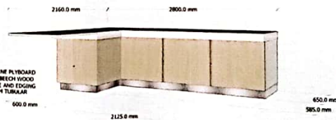
7 FACULTY OFFICE 2 COUNTER DETAIL 2(1SET) A/30 SCALE:
