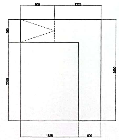
5 TOP VIEW A/31
