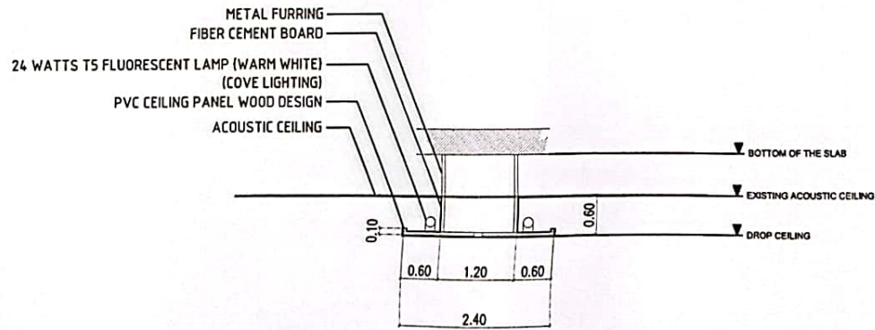
3 COVE CEILING DETAIL A/29 SCALE: 1:75M
