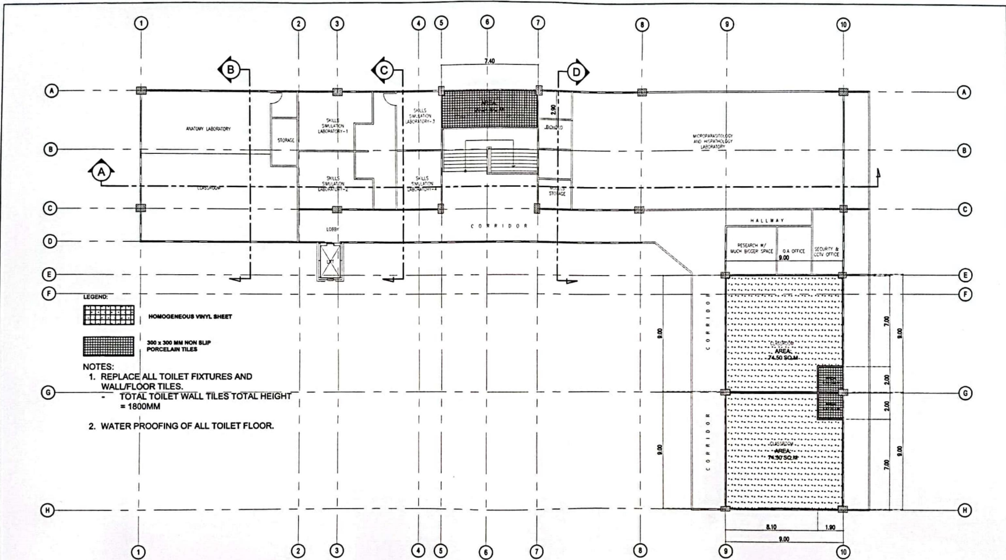
1 SECOND FLOOR (FLOOR FINISH SCHEDULE) A 26 SCALE: 1:200M
