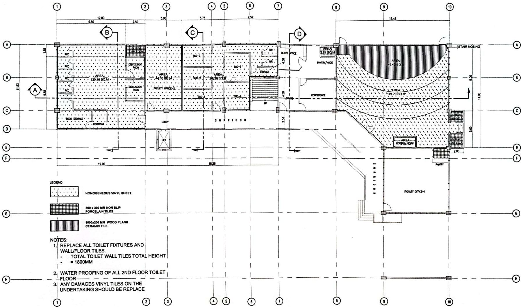
1 GROUND FLOOR (FLOOR FINISH SCHEDULE) SCALE: 1:200M
