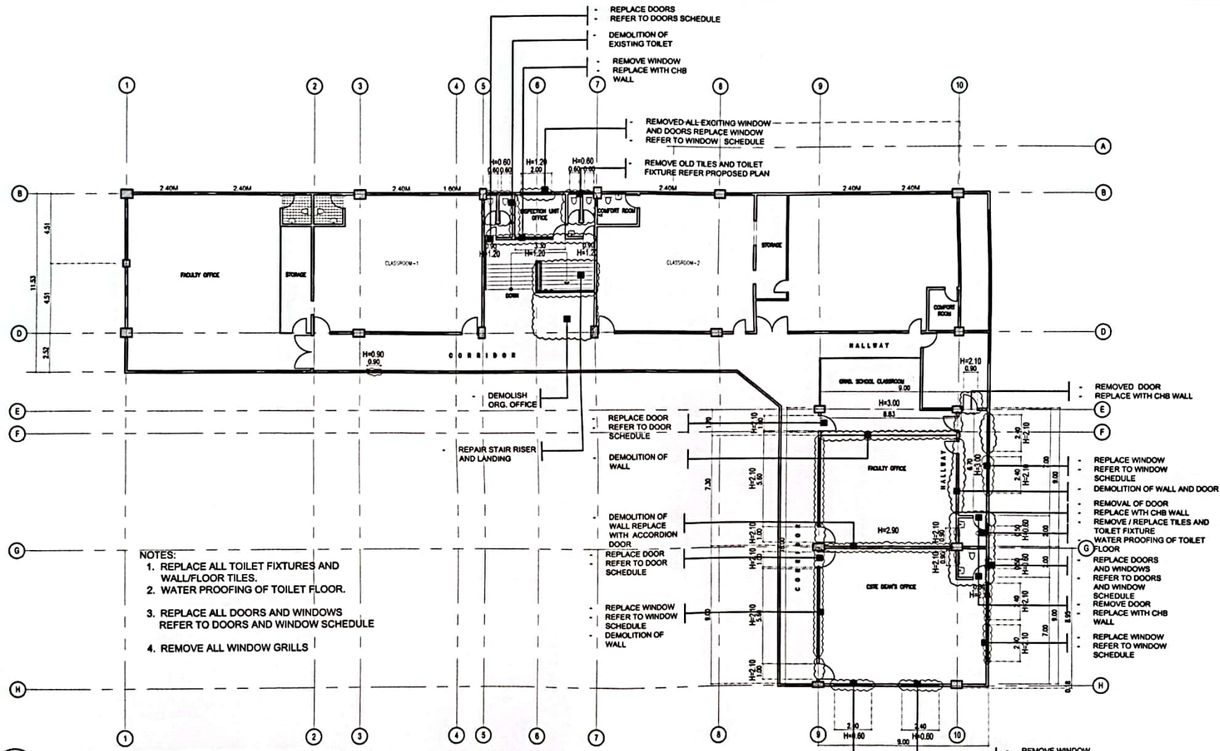
1 SECOND FLOOR DEMOLITION PLAN SCALE: 1:200M
