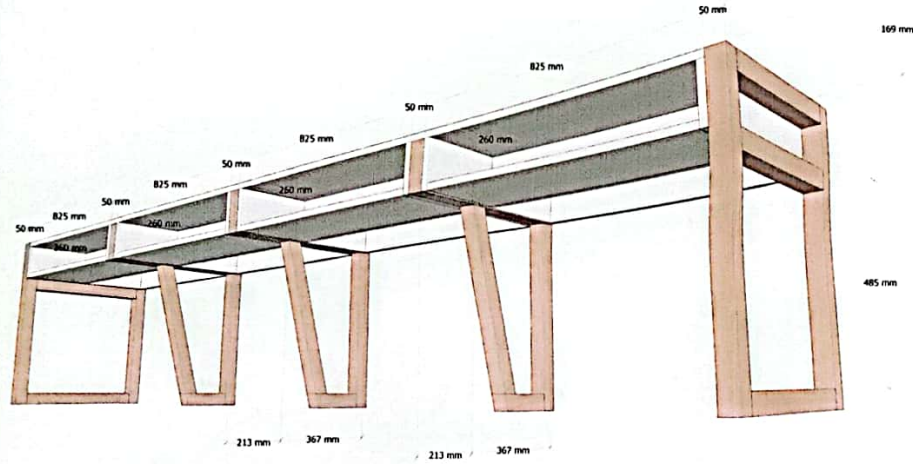
1 CLASSROOM TABLE 1 DETAIL 1 (14 SETS) SCALE: A/44
