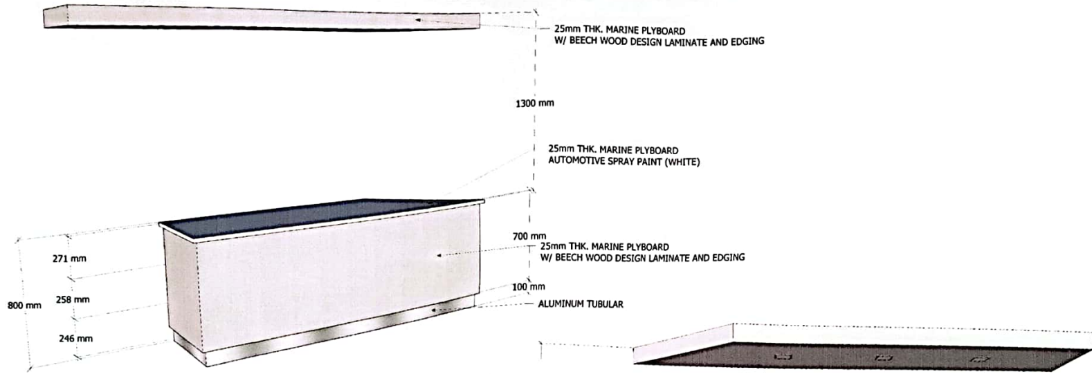
1 A.V.R. COUNTER DETAIL 1 (1 SET) A 41 SCALE:
