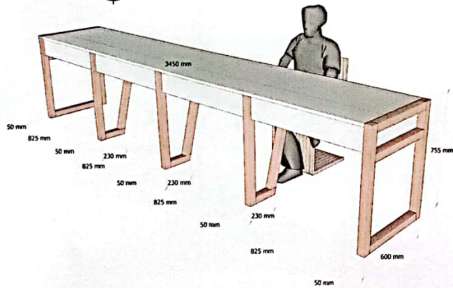
2 CLASSROOM TABLE 1 DETAIL 2 (14 SETS) SCALE: A/44
