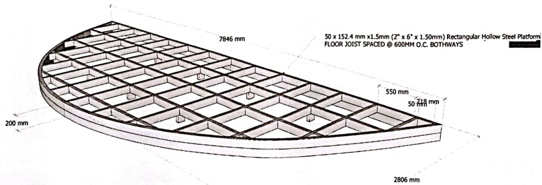
1 A.V.R. PLATFORM DETAIL SCALE:
