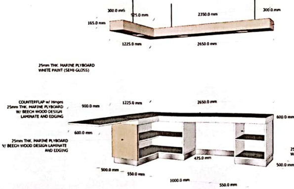
7 LIBRARY RECEPTION COUNTER DETAIL 2 (1 SET) A/31 SCALE:
