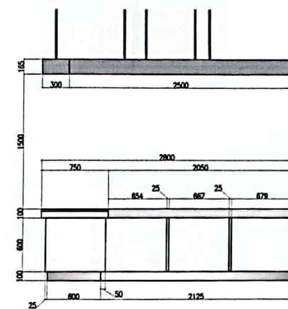
4 REAR VIEW A/30
