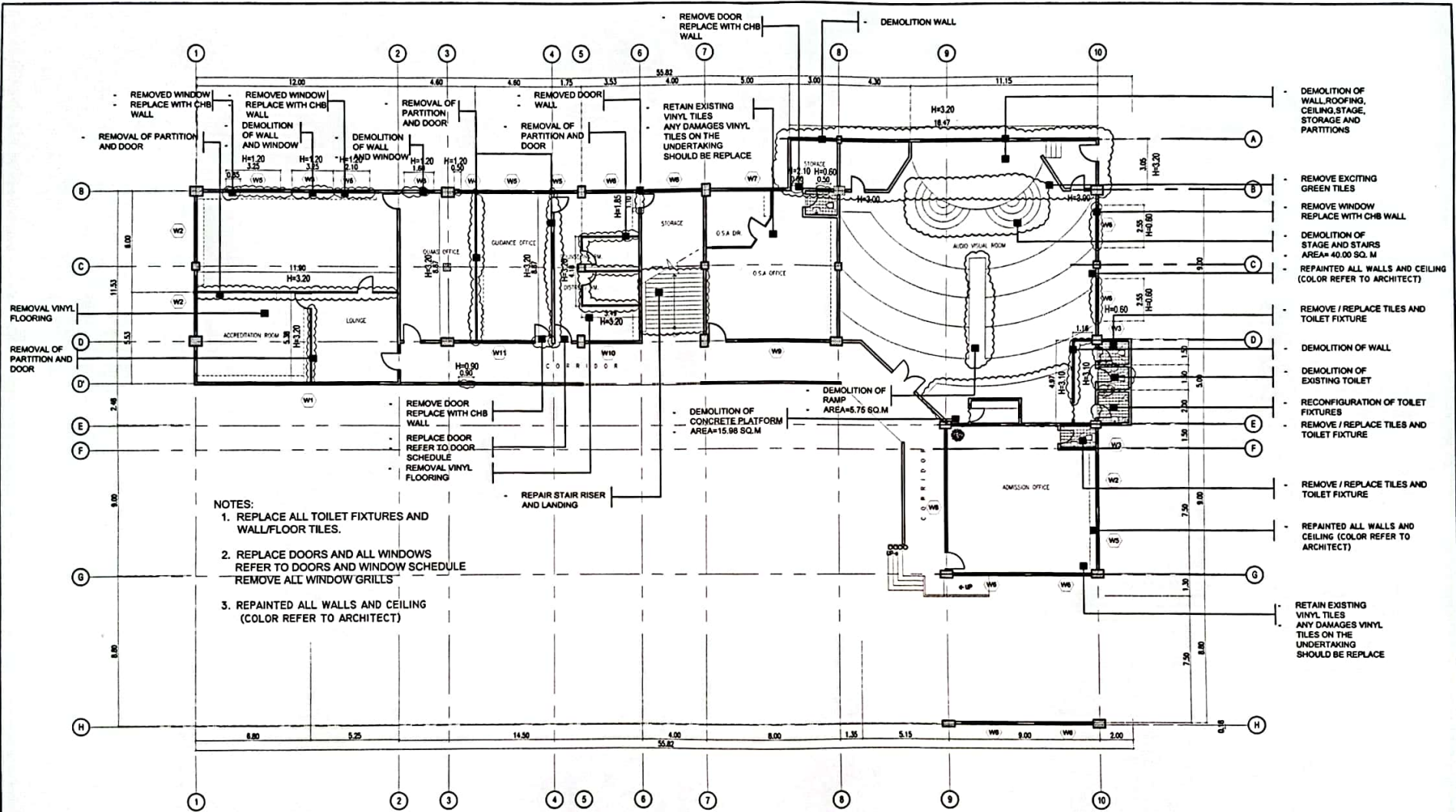
1 A/11 GROUND FLOOR DEMOLITION PLAN SCALE: 1:200M
