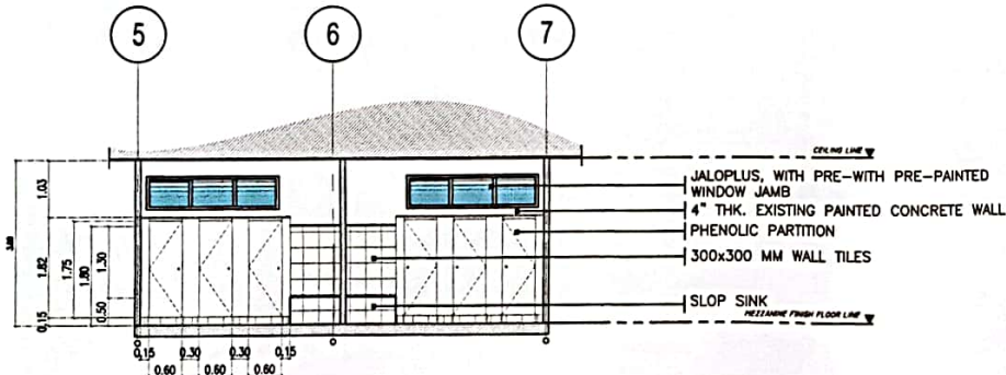
3 MALE & FEMALE TOILET MEZZANINE SECTION THROUGH B-B SCALE: 1:100M
