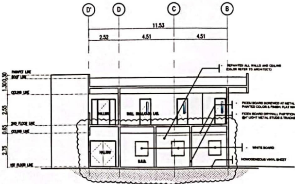
3 SECTION THROUGH "C" A/21 SCALE: 1:200M
