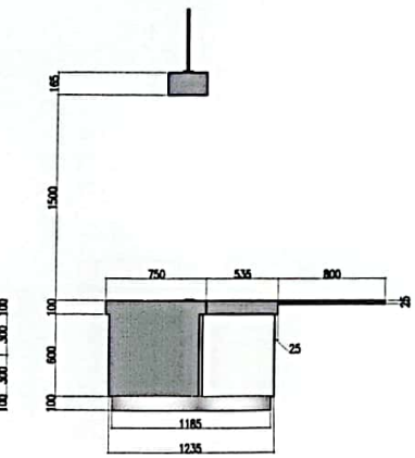
4 REAR VIEW A/B2
