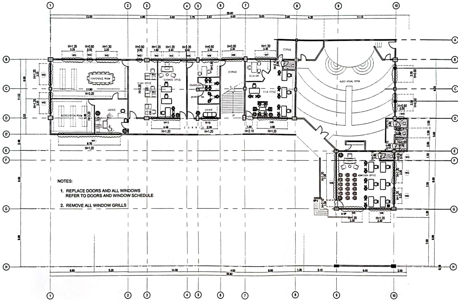
1 GROUND FLOOR DEMOLITION PLAN FOR WINDOWS AND DOORS A/12 SCALE: 1:200M
