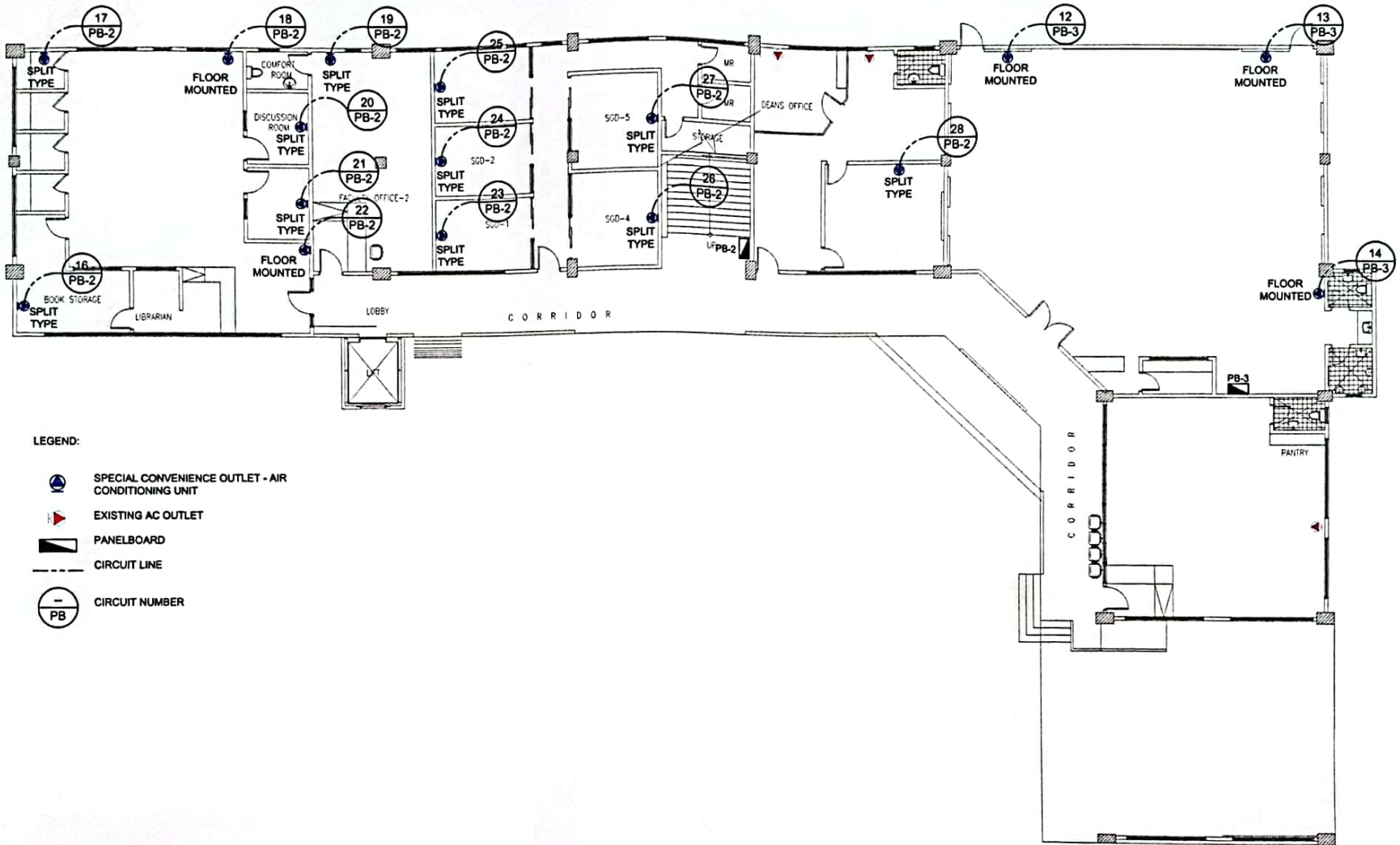
1 M 1 GROUND FLOOR MECHANICAL LAYOUT SCALE: 1:175M
