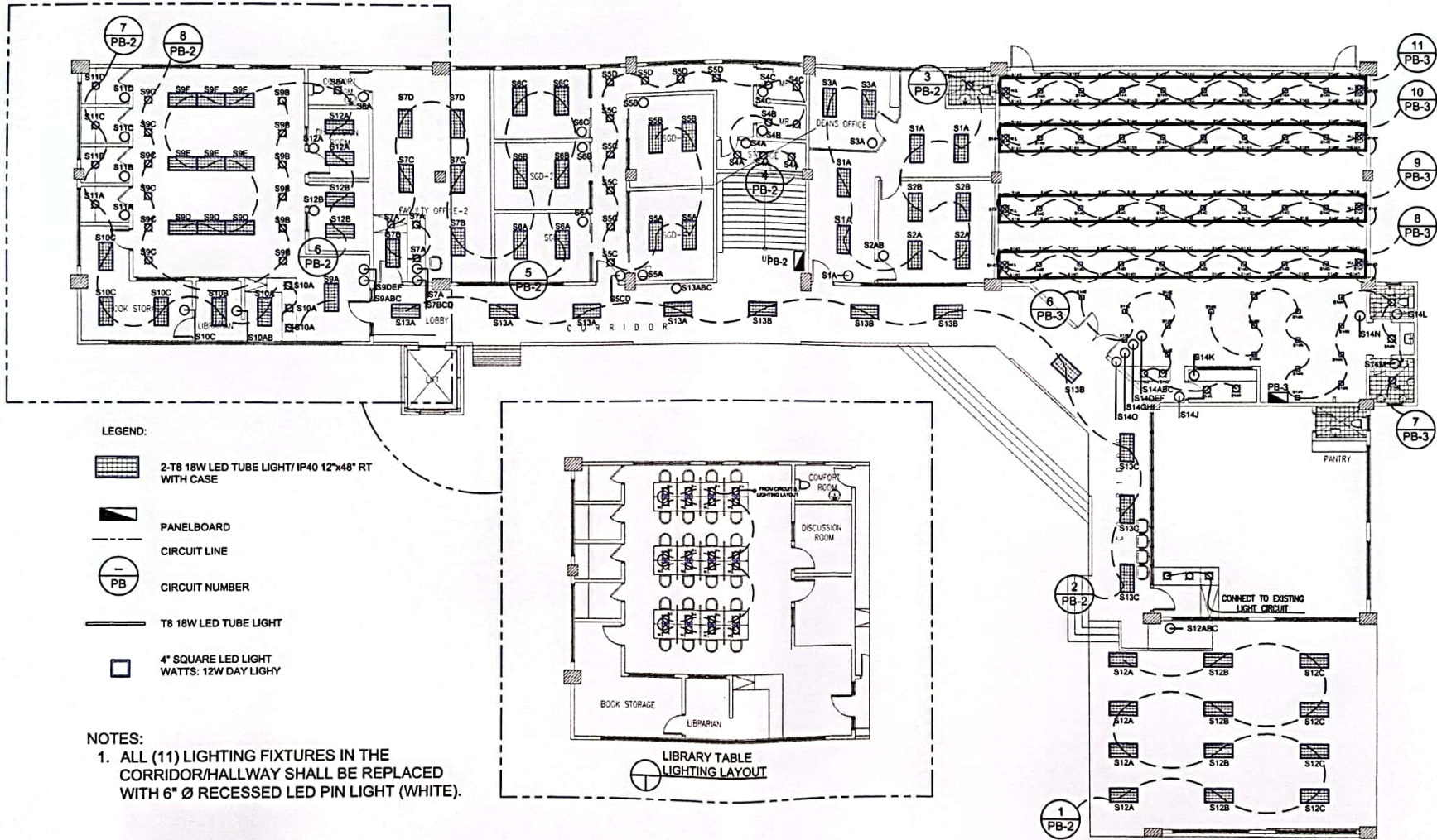
1 E 2 GROUND FLOOR LIGHTING LAYOUT SCALE: 1:175M
