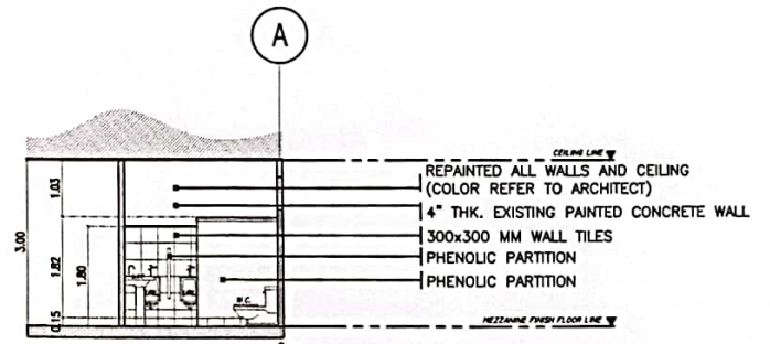
4 MALE & FEMALE TOILET MEZZANINE SECTION THROUGH C-C SCALE: 1:100M
