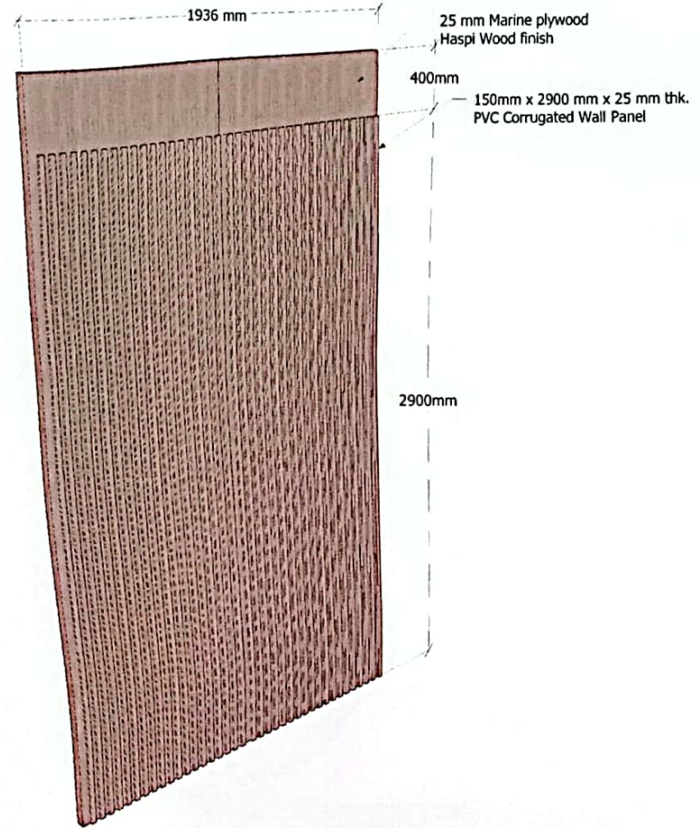
2 A.V.R. ACCENT WALL DETAIL (2 SETS) A/38 SCALE:
