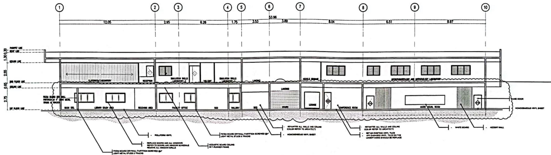
1 SECTION THROUGH "A" A/21 SCALE: 1:200M
