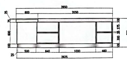
4 REAR VIEW A/31
