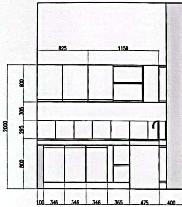
1 FRONT VIEW A/32
