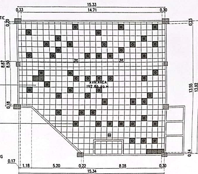
1 EXISTING A.V.R. CEILING PLAN A/29 SCALE: 1:175M
