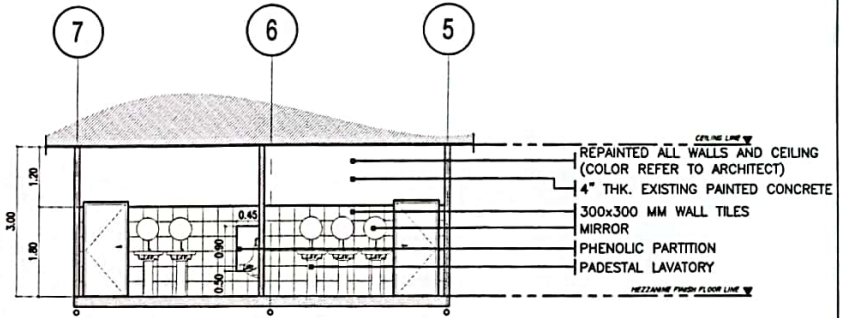
2 MALE & FEMALE TOILET MEZZANINE SECTION THROUGH A-A SCALE: 1:100M
