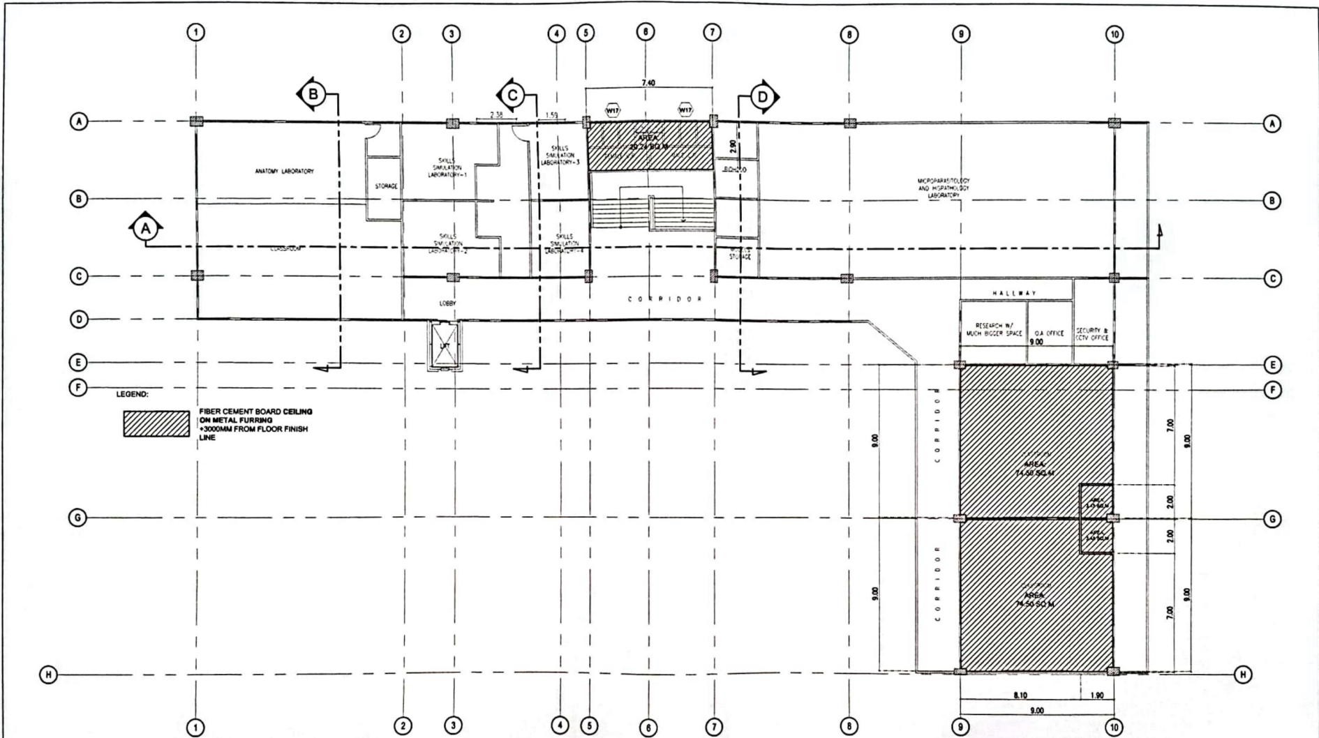
1 A/25 SECOND FLOOR REFLECTED CEILING PLAN SCALE: 1:200M
