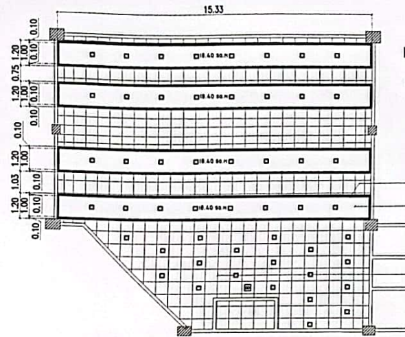
2 PROPOSED A.V.R. CEILING PLAN A/29 SCALE: 1:175M
