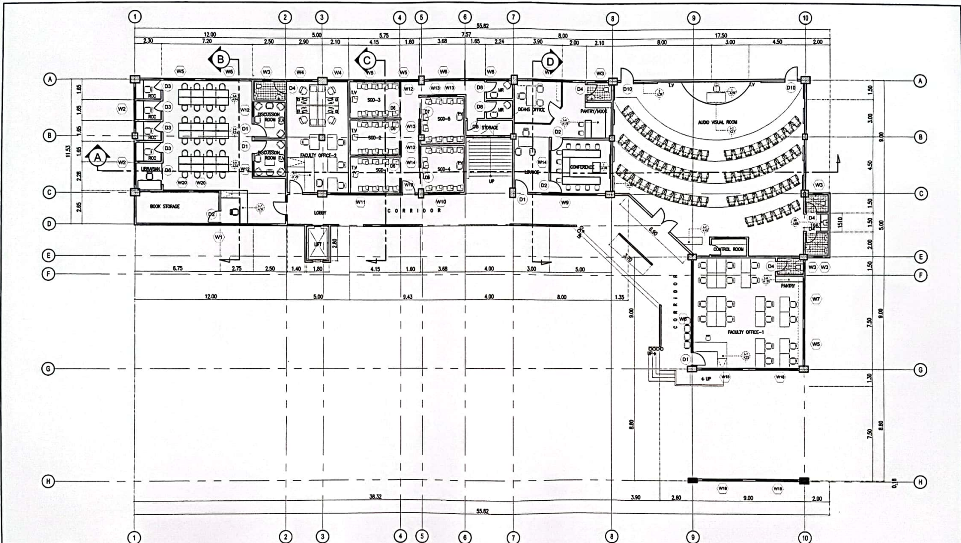
1 A/10 PROPOSED GROUND FLOOR PLAN SCALE: 1:200M
