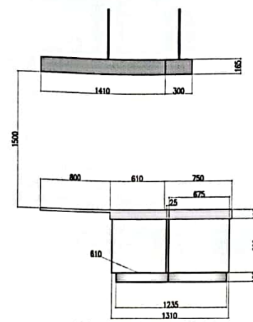
3 RIGHT SIDE VIEW A/30
