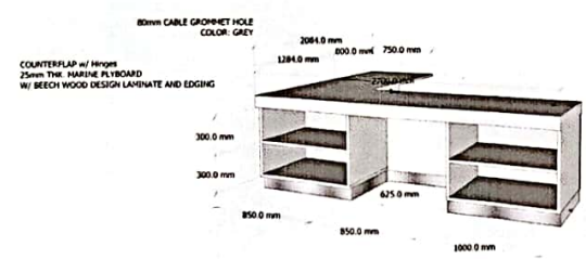
6 FACULTY OFFICE 1 COUNTER DETAIL 2 (1 SET) SCALE:
