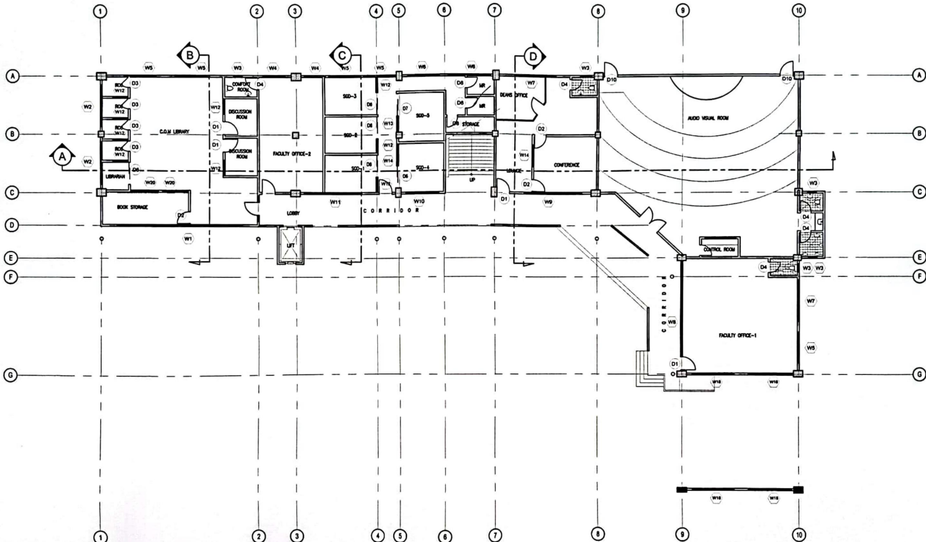
1 A/18 GROUND FLOOR SCHEDULE OF DOORS AND WINDOWS PLAN SCALE: 1:200M
