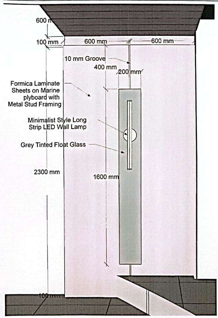
2 A.V.R LED ACCENT WALL (8 SETS) A/36 SCALE:
