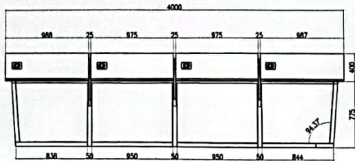
1 FRONT VIEW A/34
