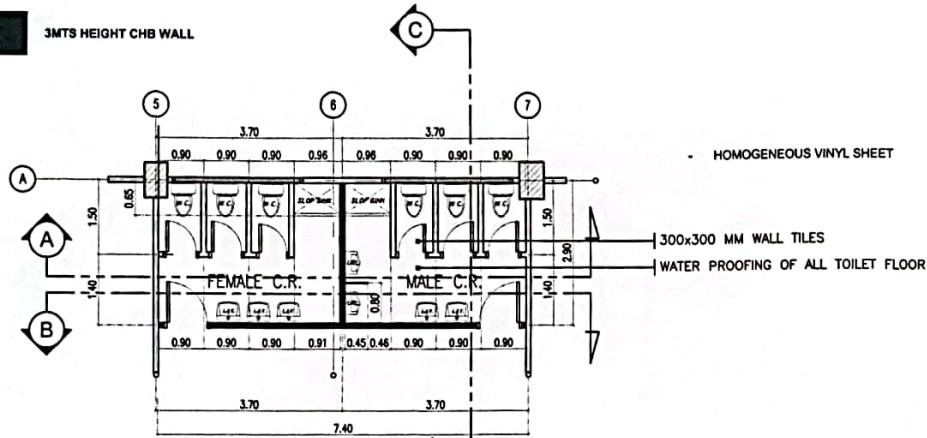
1 MALE & FEMALE TOILET MEZZANINE FLOOR PLAN SCALE: 1:100M
