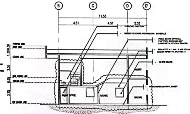
4 SECTION THROUGH "D" A/21 SCALE: 1:200M
