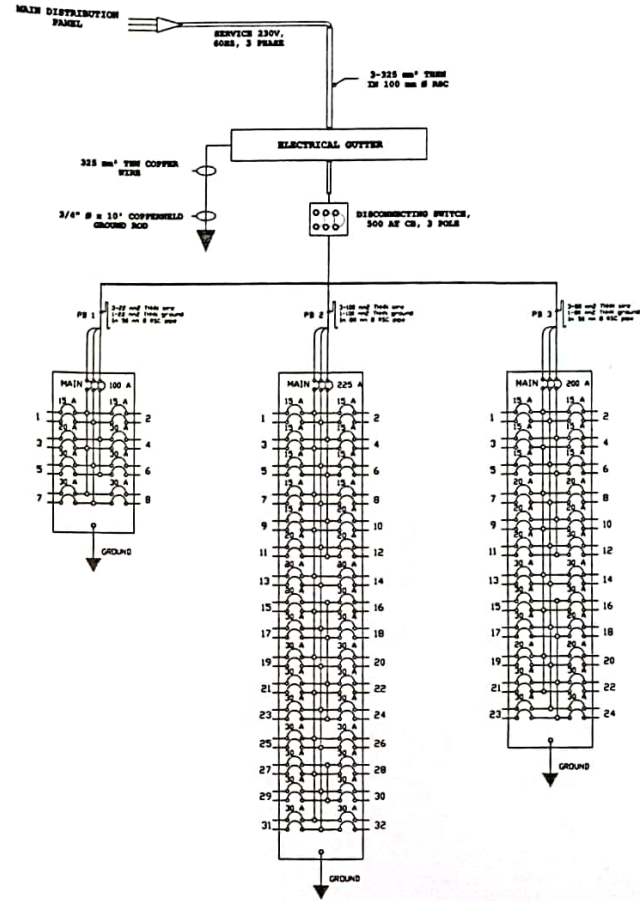
RISER DIAGRAM / SINGLE LINE DIAGRAM SCALE: NTS
