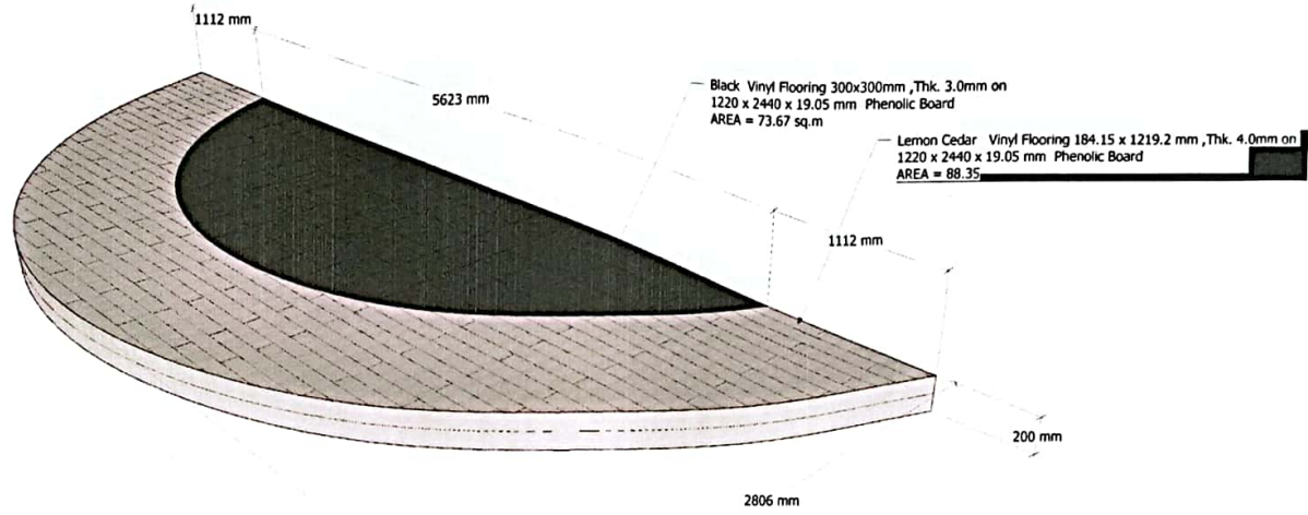
1 A.V.R. PLATFORM DETAIL SCALE:
