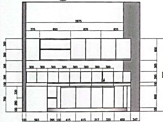
2 RIGHT SIDE VIEW A/32
