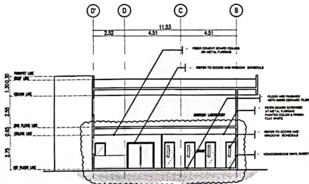
2 SECTION THROUGH "B" A/21 SCALE: 1:200M
