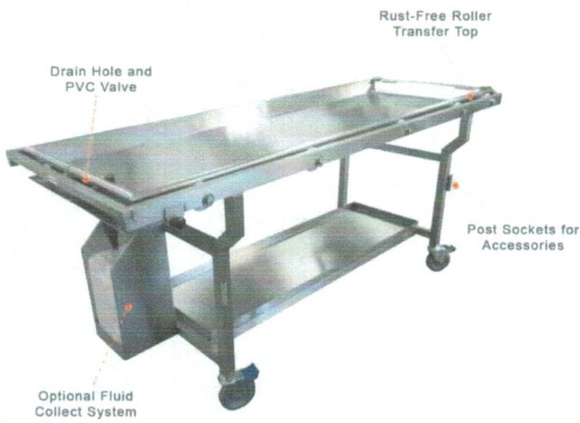
14. Standard Mobile Anatomy Table for Dissection/Cadaver Table
